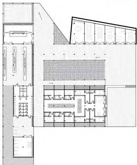
PLAN GROUND FLOOR
